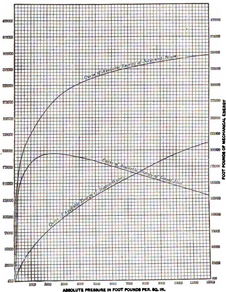
FIG. 73.—CURVE OF HEAT-ENERGY IN STEAM.
